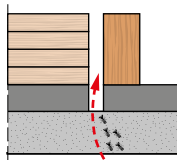
Joint traversant (retrait ou dilation)
